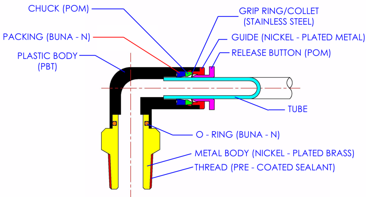
SCHEMATIC OF TYPICAL COMPOSITE FITTING CONSTRUCTION
